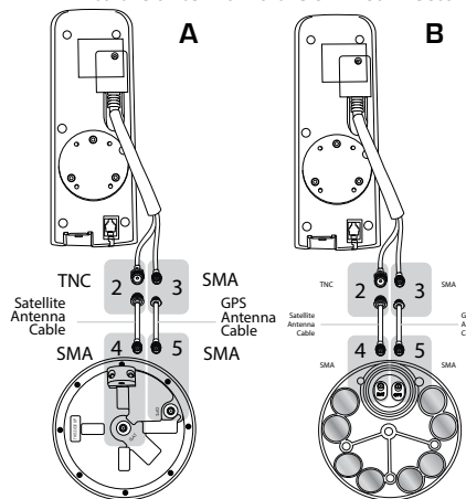
A - Connection with Fixed/Directional Antenna (Passive)
