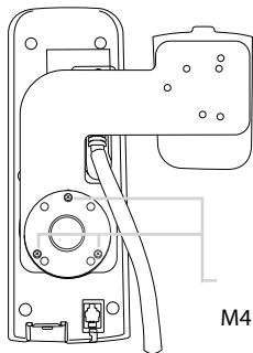
[a] Rear of IsatDock2 LITE [b] Spacer plate [c] Mounting bracket [d] RAM® base [e] 3 x M4x18 screws and washers
