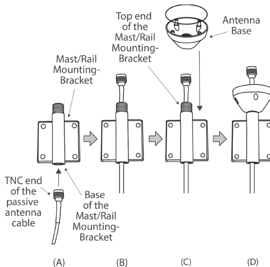
Horizontal installation
