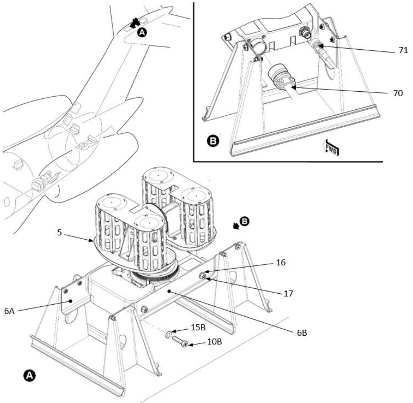
Figure 3: Assembly Installation in Vertical stabilizer tip – FOR ILLUSTRATION ONLY
