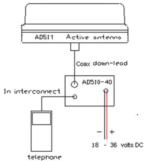
Figure 4. Schematic diagram for system connections
