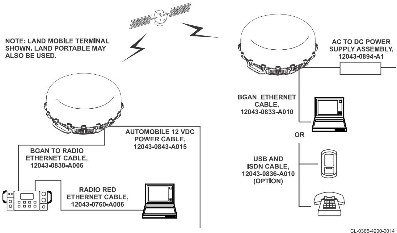
Figure 2-11. Cabling Options
