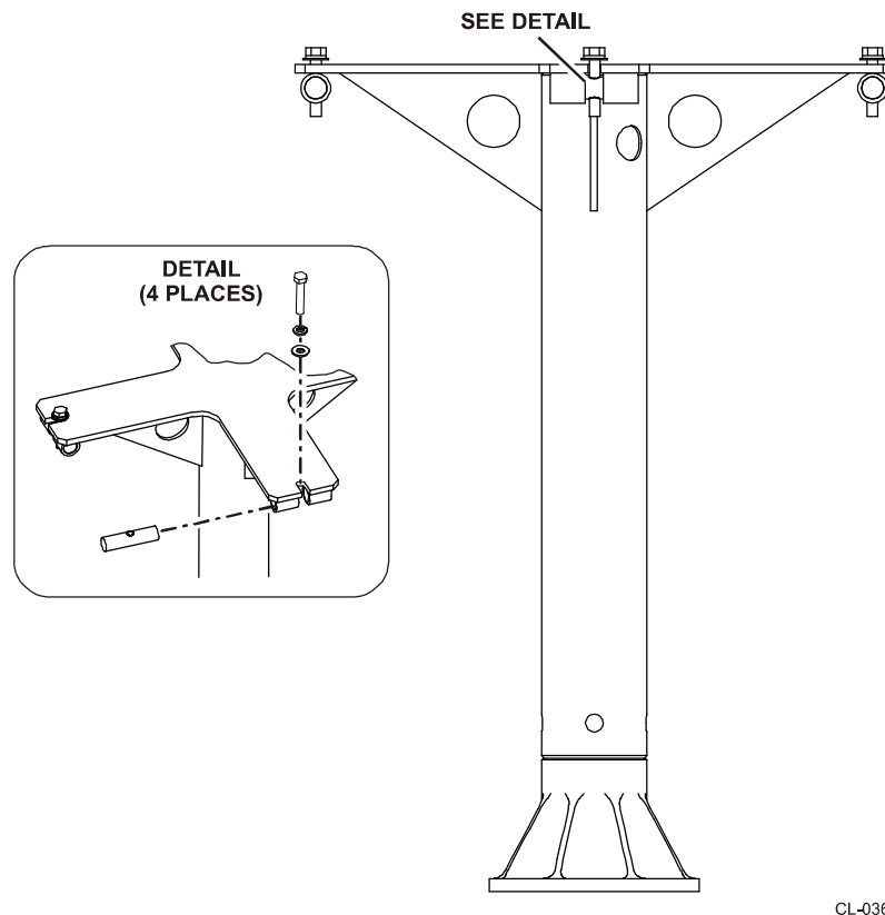
Figure 2-9. Pole Mount Option
