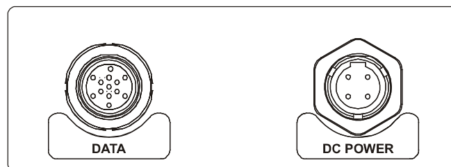
Figure 3-1. RF-7800B-VU104 Connectors
