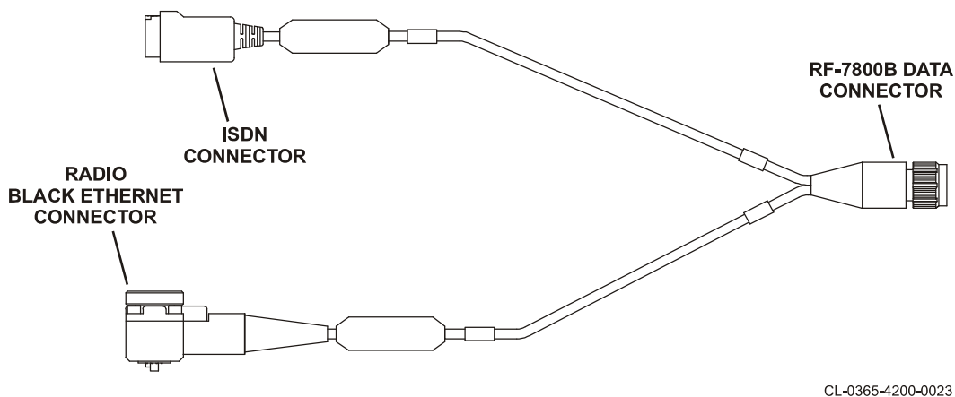
Figure 3-8. BGAN to Radio Black Ethernet and ISDN Cable, 12043-0831-A006 (Optional)
