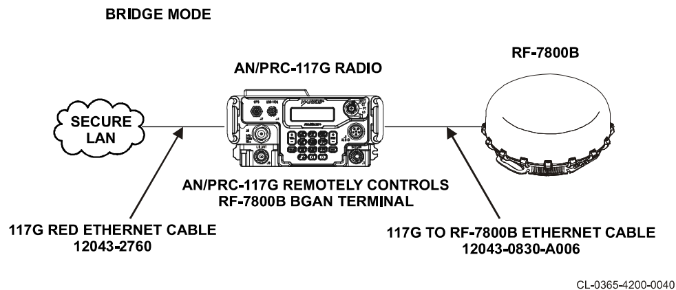
Figure 4-3. Bridge Mode Connections
